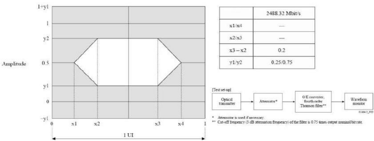
Figure 1 Transmitter Eye Mask Definitions and Test Procedure
