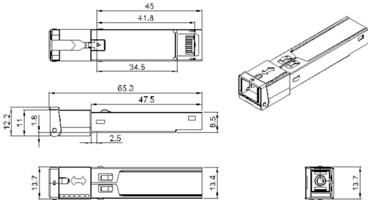
Figure 8 Package Outline
